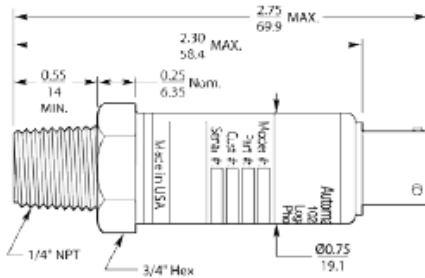
4 PIN Bayonet
